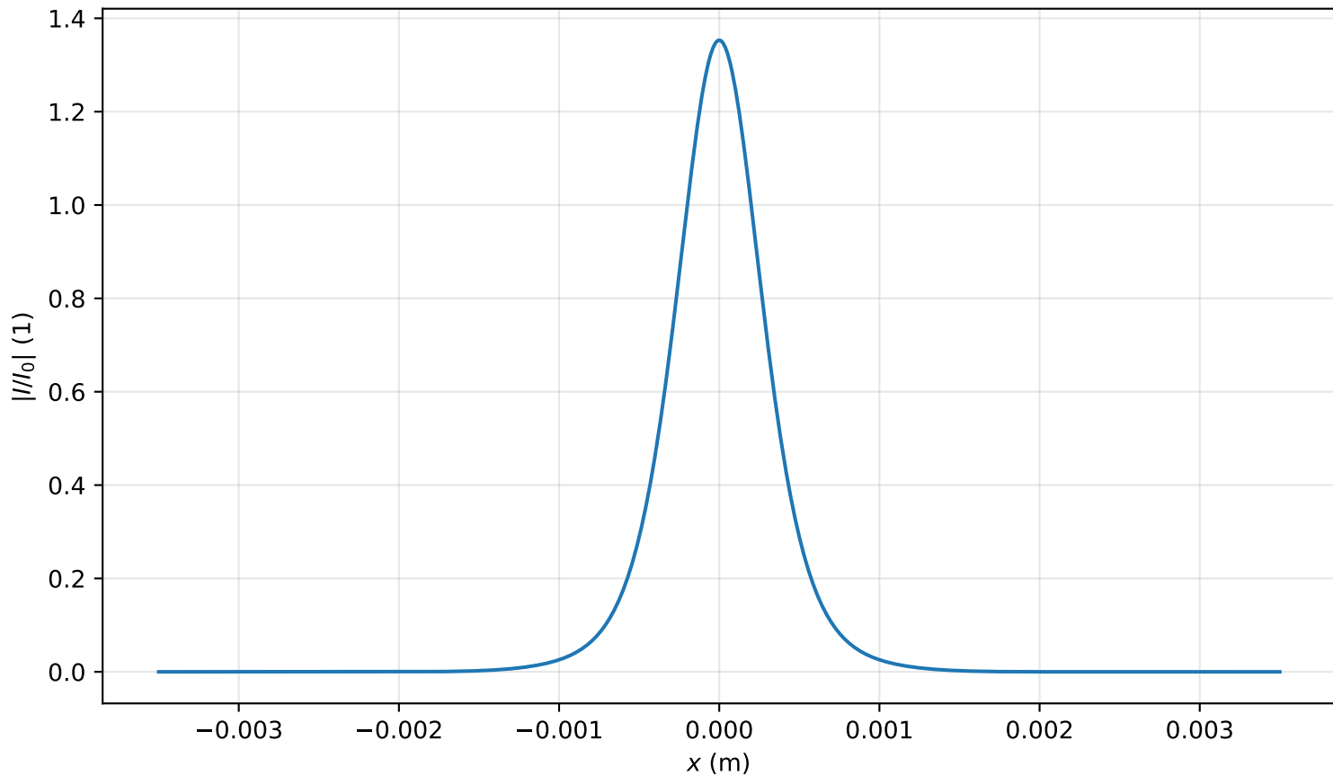
Intensity profile I(x, y = 0, z = 1.672m)/I_0 , P_{in}=0.8P_{cr} , artificial time
